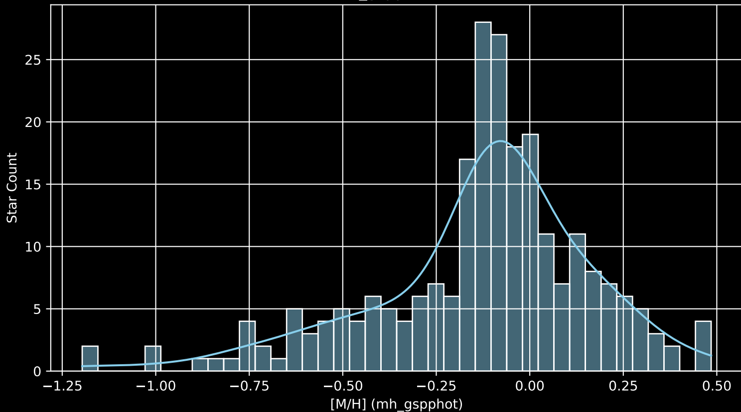
APOGEE DR17 Field: [296+12 [M/H] (mh_gspphot) (n= 242)
