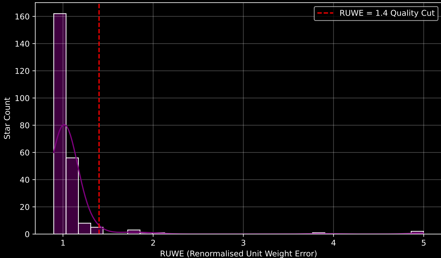
GAPOGEE DR17 Field [296+12] RUWE Distribution (n= 239)
