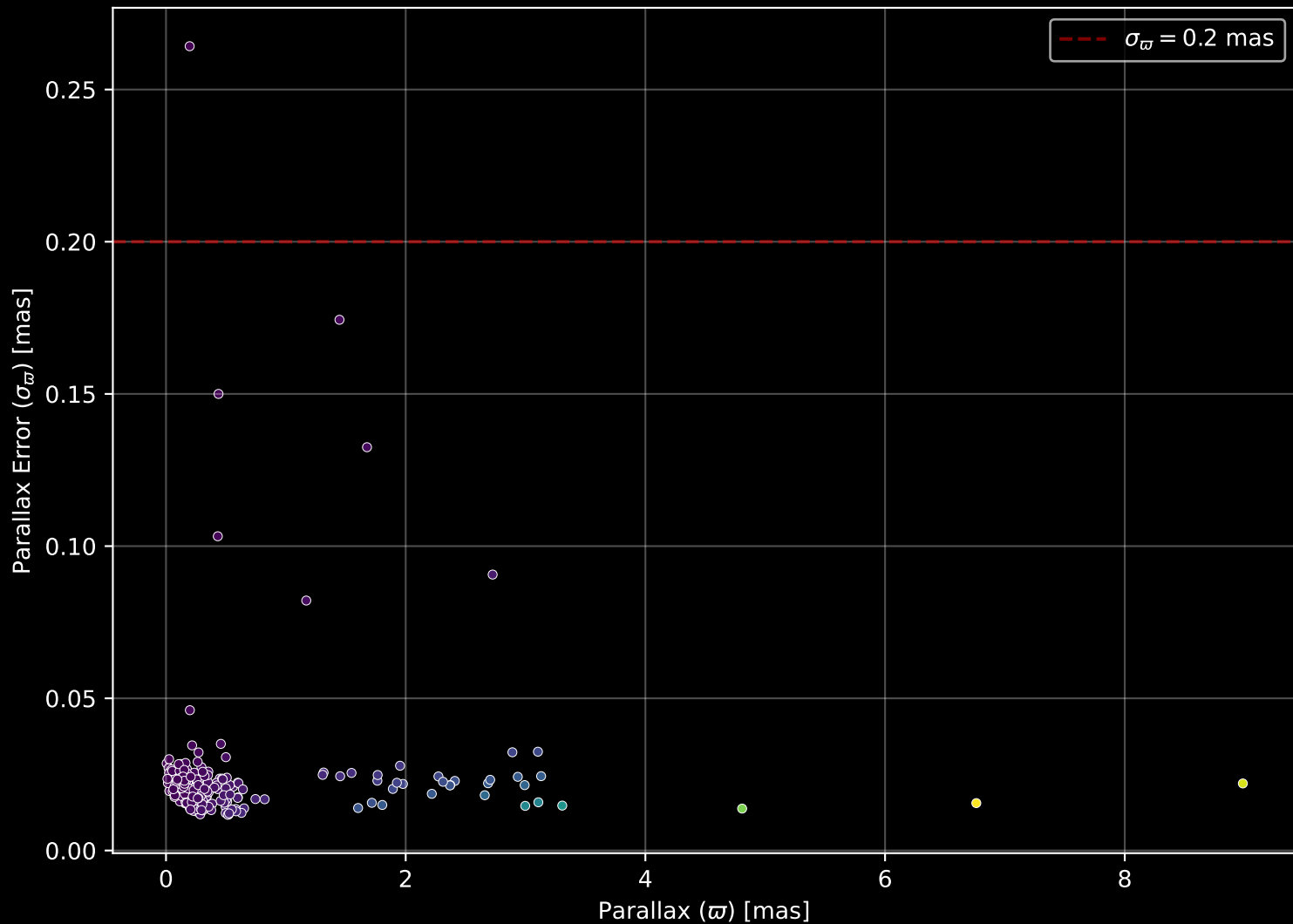
APOGEE DR17 Field: [296+12] Parallax Quality (n= 243)
