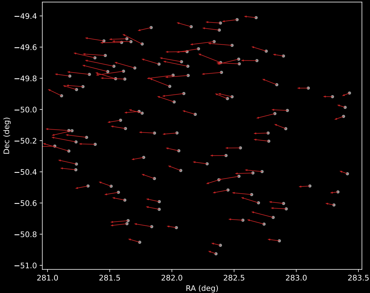
APOGEE DR17 Cluster 6 Proper Motion Vectors (n=109)
