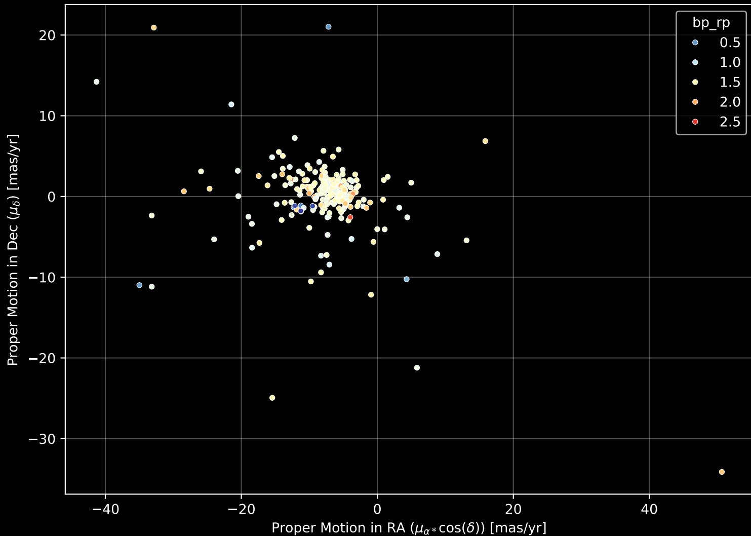
APOGEE DR17 Field: [296+12] Proper Motion Diagram (n= 243)
